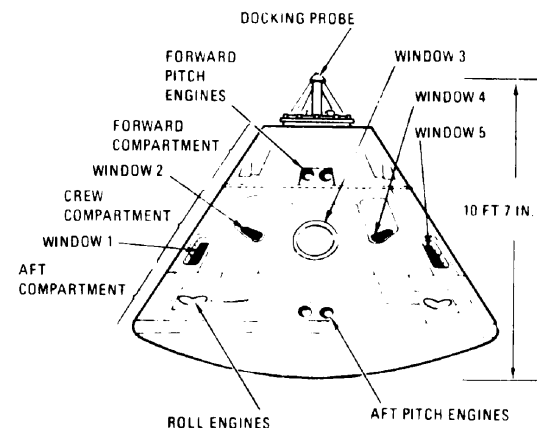
CM General Arrangement
