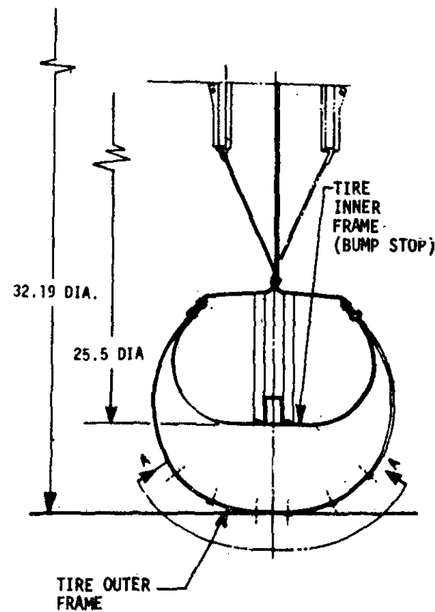
LRV WHEEL
